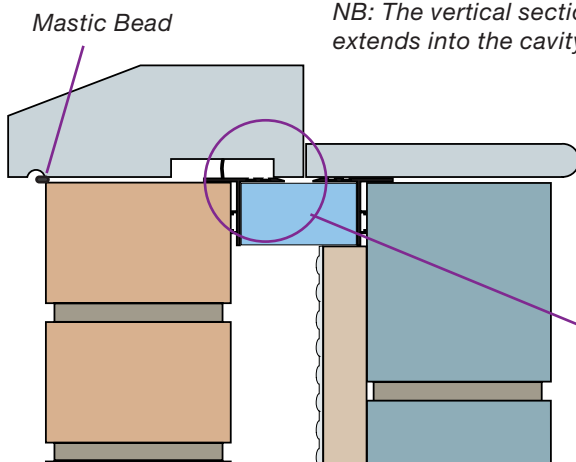
This detail shows how the flexible seal would prevent further water ingress if the mastic seal failed.
