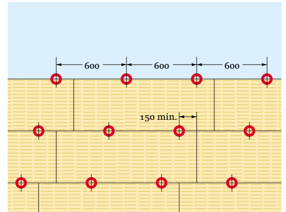
Figure 2 Between slabs
