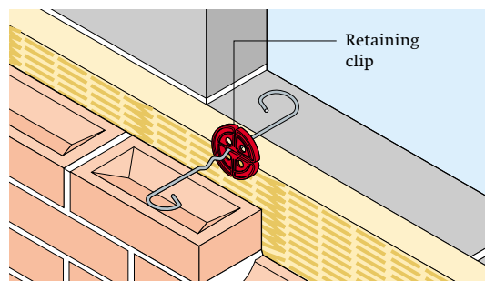
Fig 4 Between slabs
