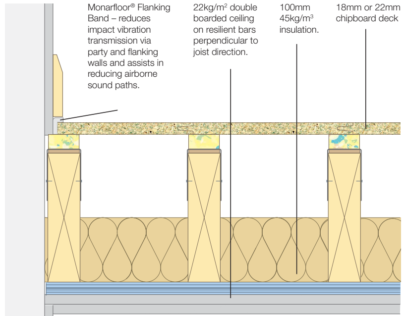
Monarfloor® Acoustic Strip on solid timber joists with a resilient bar ceiling.
