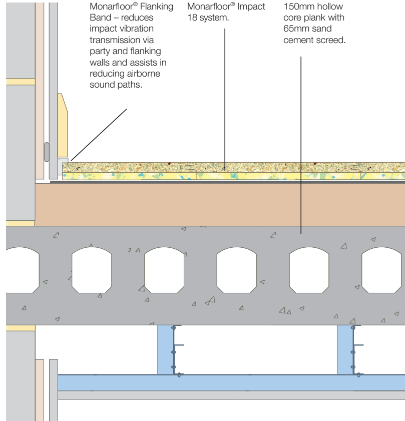
Monarfloor® Impact 18 over 65mm sand/cement screed and 150mm precast concrete plank (Robust Details E-FC-1 with FFT4/FFT5 Floating Floor).
