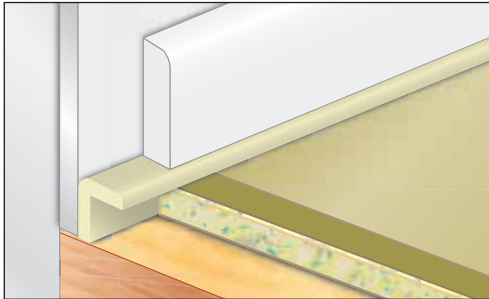
Monarfloor® Impact 18 over 65mm sand/cement screed and 150mm precast concrete plank (Robust Details E-FC-1 with FFT4/FFT5 Floating Floor).
