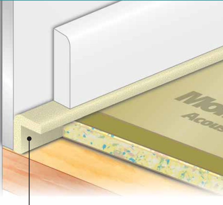
Monarfloor® Angled Flanking Band
