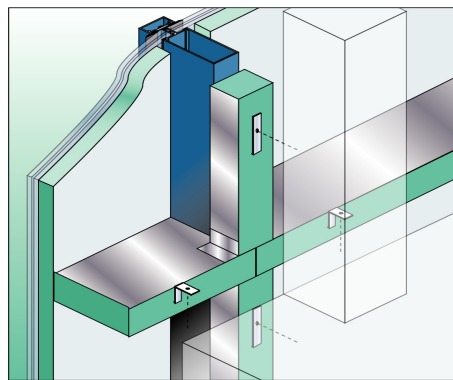
Fig 1: Horizontal & Vertical CW fire stops at curtain wall
