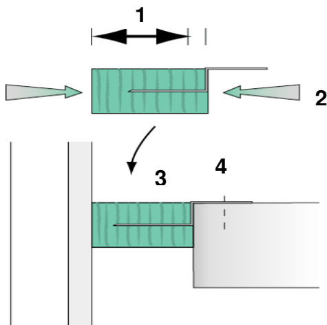
Fig 3b Horizontal CW Fire and smoke stop assembly
