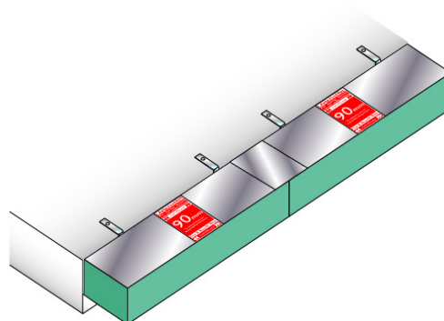
The cut strips are inserted within the cavity with the fixing brackets simply located over the slab edge. Note! The brackets should be mechanically fixed to slab where void sizes exceed 400mm
