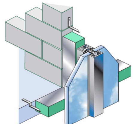
Fig 2: Horizontal & Vertical CW fire stops at party floor and wall
